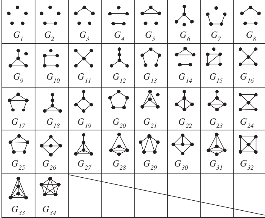
Figure 6: All graphs of order 5 [2].
