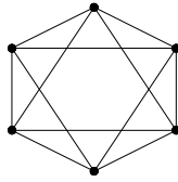
Figure 2: C_4 -regular graph.
