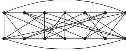
Figure 7: (P_3 \cup P_2) -regular graph.
