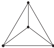
Figure 1: C_3 -regular graph.
