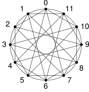
Figure 8: C_6 -regular graph.
