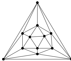
Figure 3: C_5 -regular graph.
