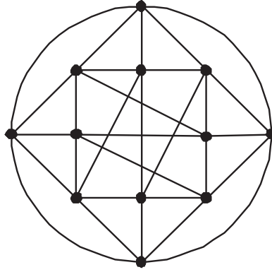
Figure 5: P_5 -regular graph.
