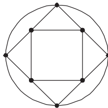
Figure 4: P_4 -regular graph.
