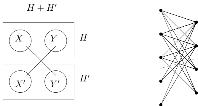
Figure 2.2: The bipartite sum and an example K_{3,2} + N_{2,2}
